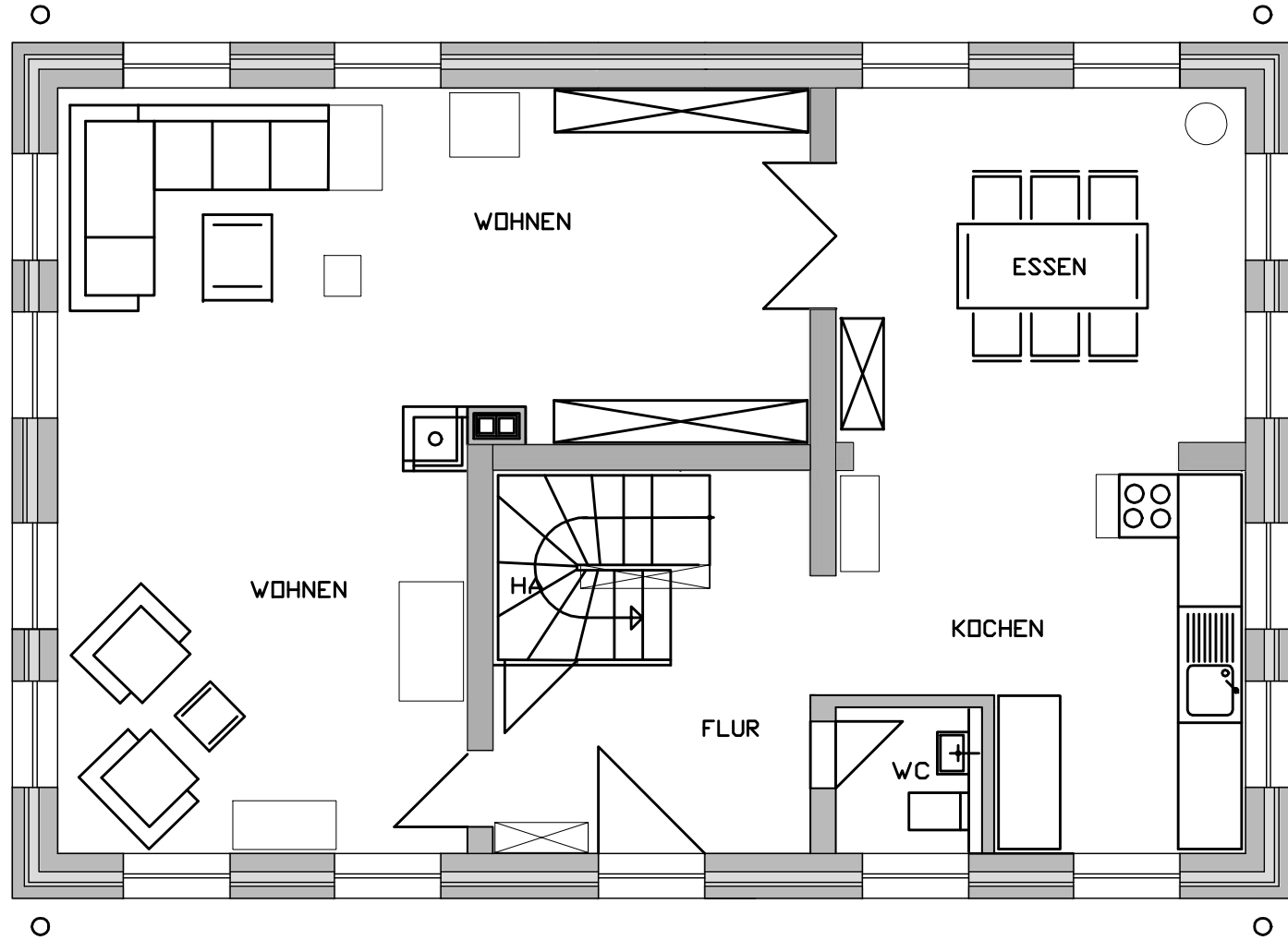
GRUNDRISS EG TARA'S Hus
